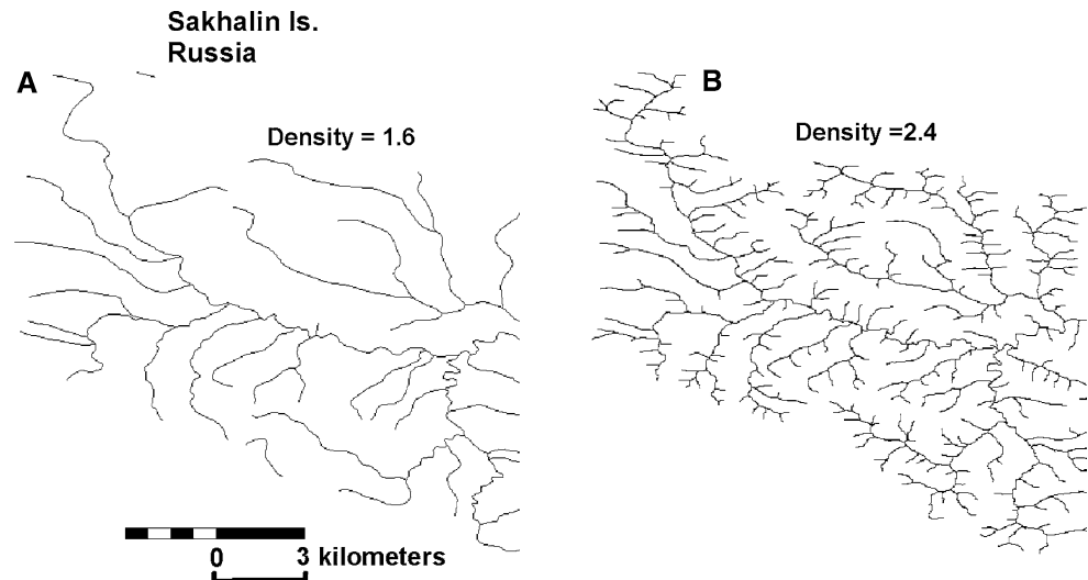
Fig. 3 a The Russian cartographic stream layer for Sakhalin Island has a low stream density (Table 2). b A synthetic stream layer built using 30-m DEMs has a higher channel density but still comparatively low because of the low-resolution DEMs (Table 2)
