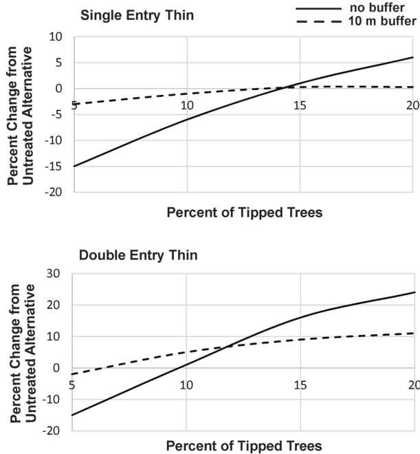
Fig. 5 Negative values refer to wood volume that is less than the no treatment and positive values refer to wood volumes greater than the no treatment. To completely offset the loss of in-stream wood due to thinning (single entry) would require a 14 % rate of tree tipping; adding a buffer reduces the effectiveness of tree tipping. In the double entry thin, a 6 and 10 % rate of tree tipping would be necessary to completely offset the loss of in-stream wood due to thinning with and without a buffer respectively
